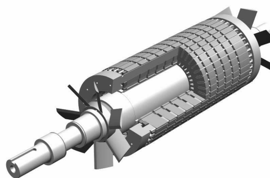
FIG. 4 - 3D CuBar Rotor Cutaway View
