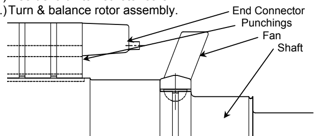
FIG. 1 - ADC Rotor Cutaway View
